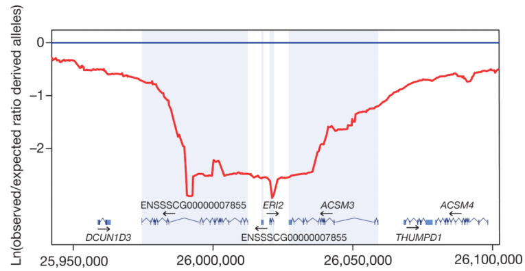
Figure 4. Putative selective sweep region around the ERI2 gene on SSC3 The y axis shows the log-transformed value of the ratio for the observed/expected derived allele frequency using a sliding window at a bin size of 50,000 bp. The x axis shows the position on SSC3 in base pairs.
